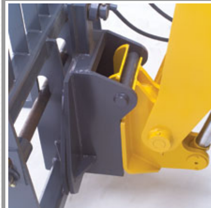
The Dynattach® Quick Carriage Release System allows for quick attachment changes. The operator does not have to leave the
